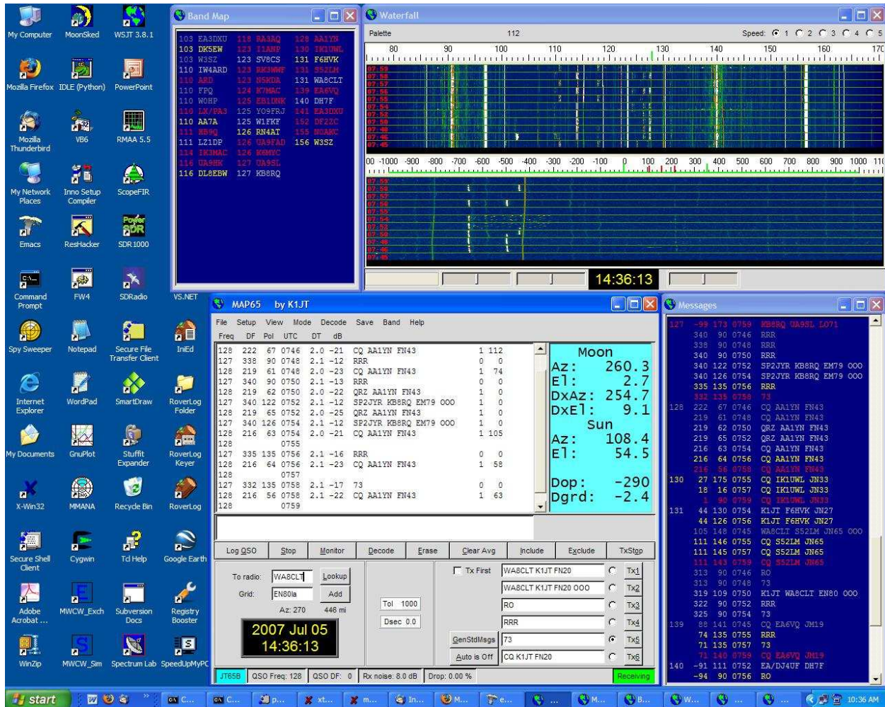
Figure 1. MAP65 screen shot after receiving 11 minutes of wideband data recorded during the 2006 ARRL EME contest at 144 MHz.
