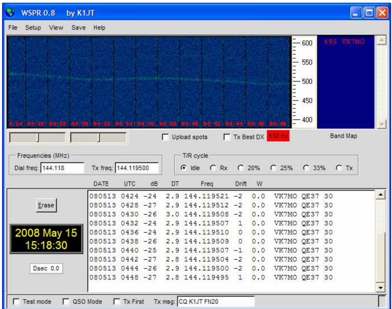
Figure 3. Screen shot showing the WSPR signal of VK7MO being received at K1JT via 144 MHz EME.
